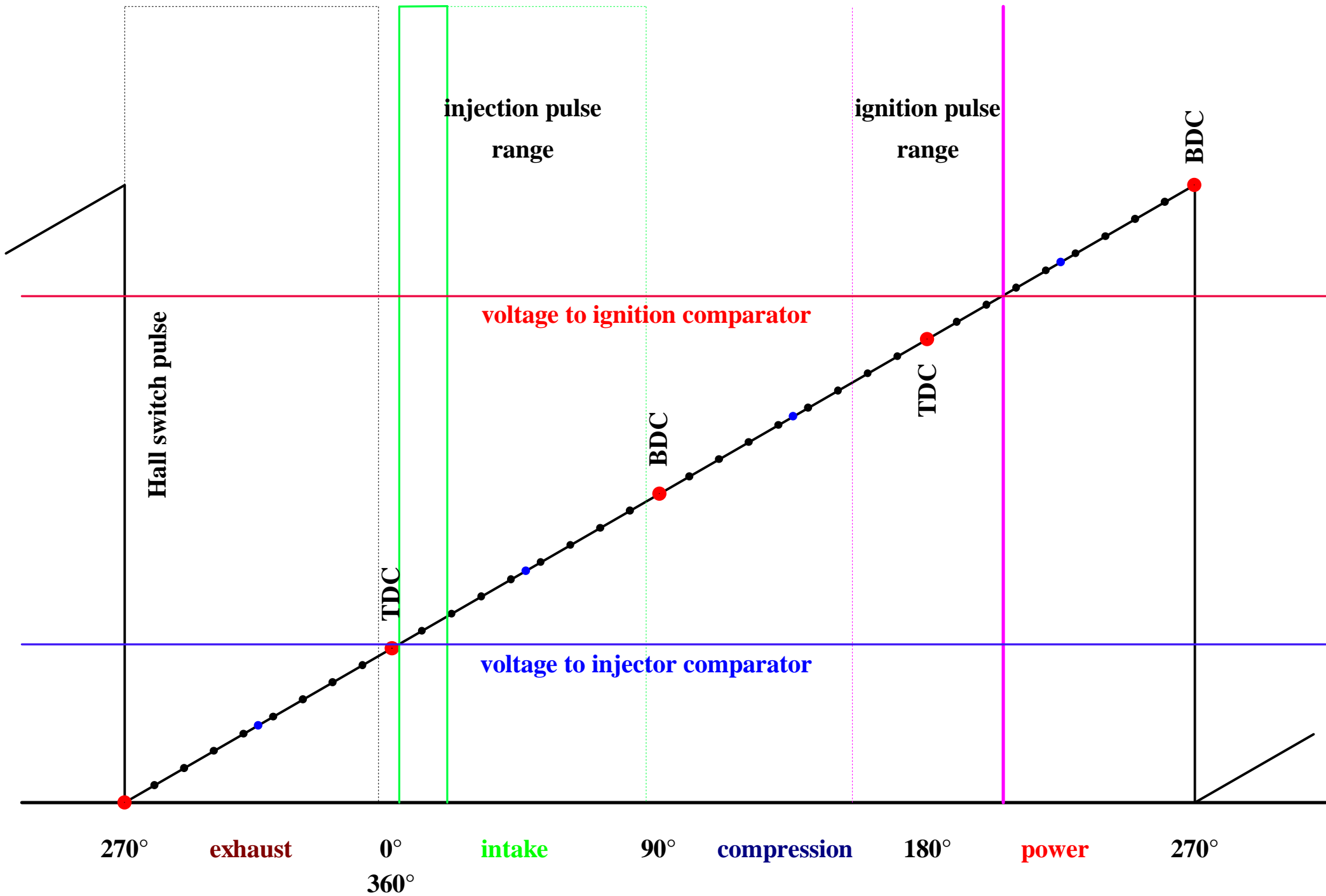
4 stroke engine timing cycle saw tooth
